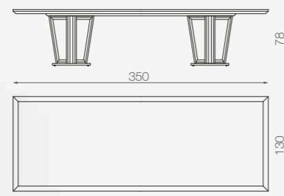
350 X 130 X 78 CM
