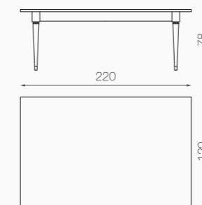
220 X 120 X H 75 CM
